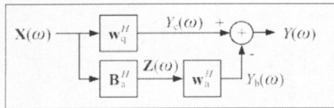
Fig. 2. Microphone array processing
