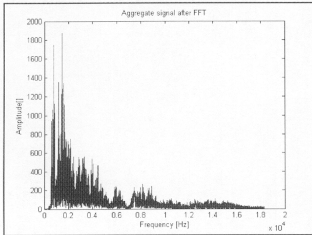
Fig. 8. Spectrum of aggregate signal after Fast Fourier Transformation
