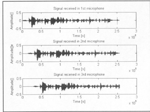
Fig. 5. Sound signals received from microphone array
