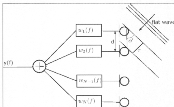
Fig. 1. Microphone array processing
