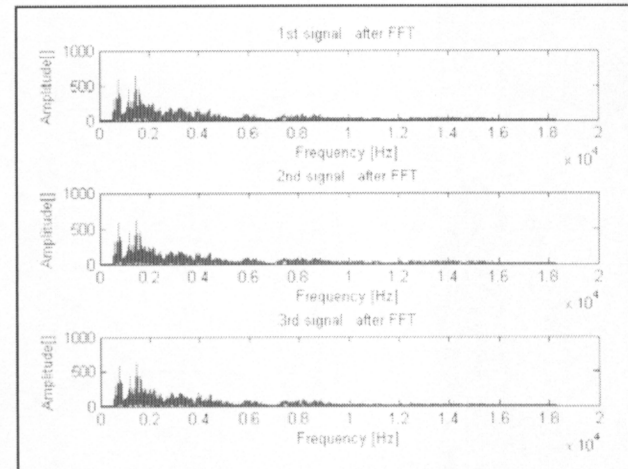
Fig.7. Sound signals spectrum applying Fast Fourier Transformation
