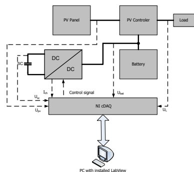
Fig.1 Block diagram of the stand for testing
