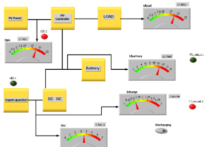
Fig.2 Front panel of the virtual instrument – control system
