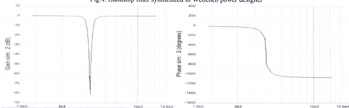
Fig. 5. Gain and phase in frequency domain for the bandstop filter from Figure 4, obtained in Webench Power Designer tool
