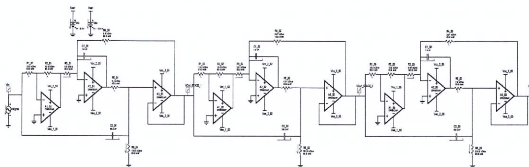
Fig.4. Bandstop filter synthesized in Webench power designer
