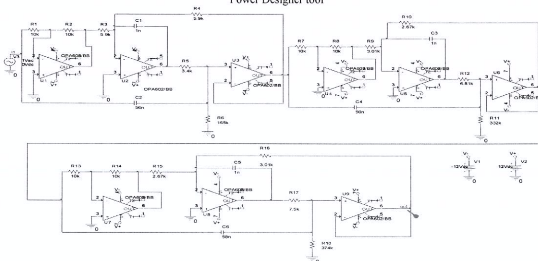
Fig.6. Electrical circuit of the Bandstop filter from Fig.4 in ORCAD Capture 16.6
