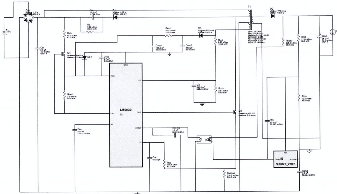
Fig. 9. Unique design solution for the SMPS for a notebook in Webench Power Designer
