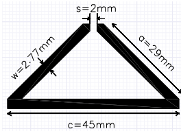
Fig.2 Triangular open loop resonator used in the simulations tuned on 811MHz
