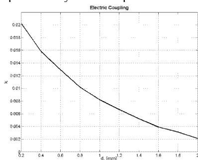
Fig.3 Coupling coefficient for electrically coupled resonators
