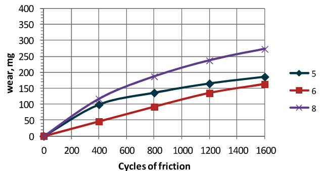
Figure 6. Dependence of the wear on the number of cycles of abrasion for coatings deposited using cored wires of the group II
