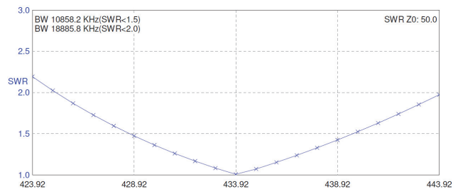
Fig. 5. SWR behaviour in the working frequency range
