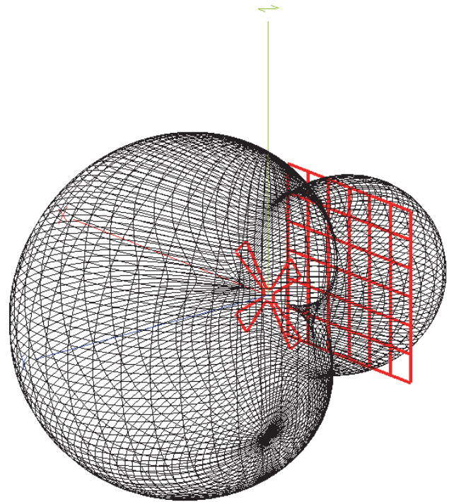
Fig. 4. 3D radiation pattern of optimized X-pol antenna
