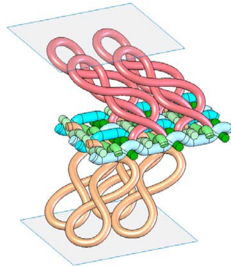
b) General appearance of the geometric model
