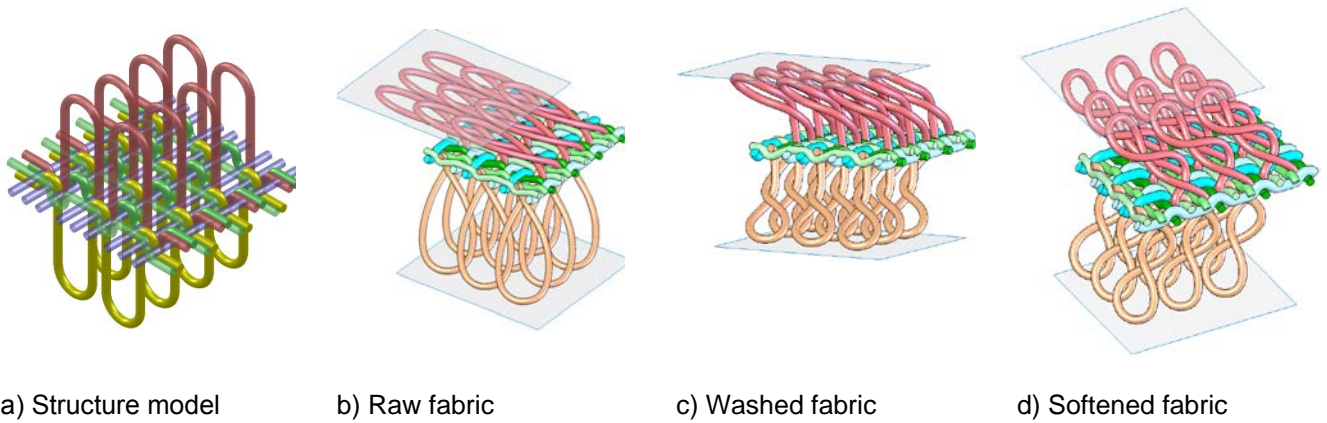
Fig.2 Geometric models of terry fabric – common type
