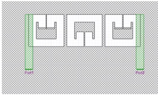
Fig. 8. Topology of the synthesized three resonator Chebyshev filter
