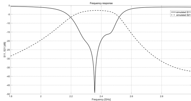
Fig. 9. Simulated narrowband frequency response of the synthesized filter.
