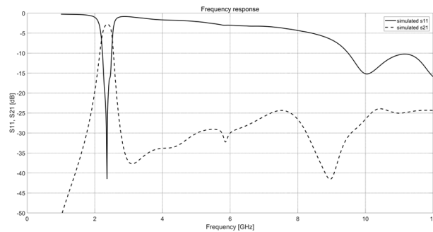
Fig. 10. Simulated wideband frequency response of the synthesized filter
