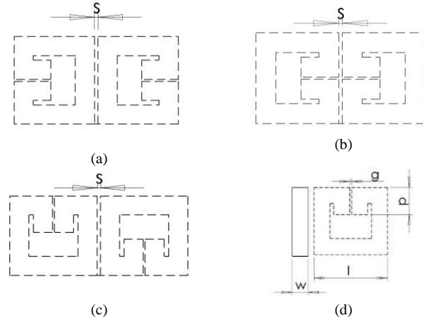
Fig. 3. Coupling topologies of miniaturized hairpin DGS resonators: (a) electric, (b) magnetic, (c) mixed, (d) external quality factor
