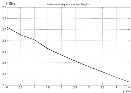
Fig. 2. Dependence of the resonant frequency of the coupled lines length
