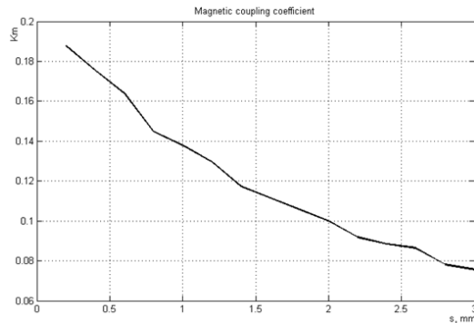
Fig. 5. Coupling coefficient as function of the separation between the resonators for the magnetic coupling
