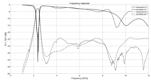
Fig. 13. Measured and simulated wideband frequency response of the synthesized filter
