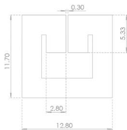
Fig. 1. Dimensions of the DGS resonator tuned to f_0=2.4\text{GHz}
