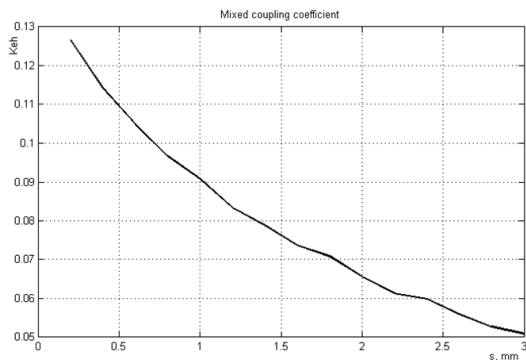
Fig. 6. Dependence of the coupling coefficient as a function of the separation between the resonators for the mixed coupling
