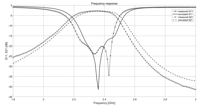
Fig. 12. Measured and simulated narrowband frequency response of the synthesized filter
