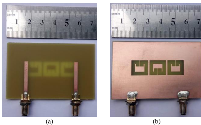
Fig. 11. Fabricated PCB of the synthesized three resonator Chebyshev filter: (a) top layer, (b) bottom layer
