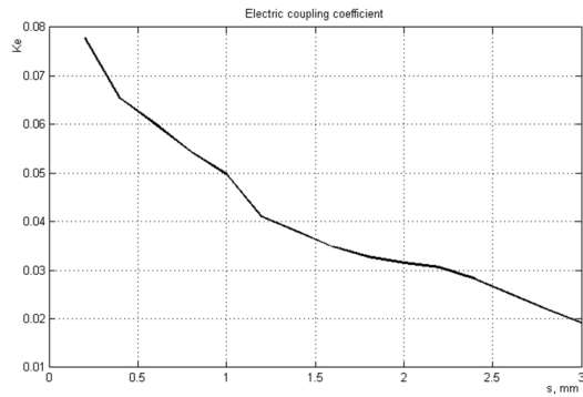
Fig. 4. Coupling coefficient as function of the separation between the resonators for the electric coupling
