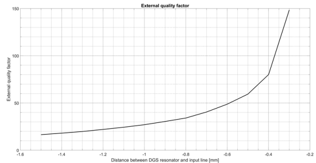
Fig. 7. Dependence of the external coupling as a function of the position of the input/output microstrip line
