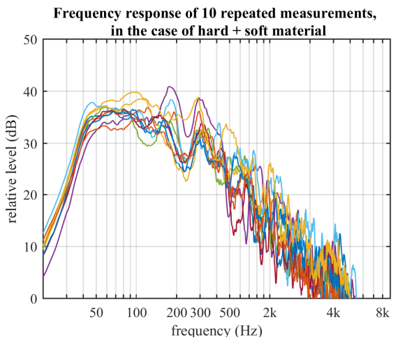
Fig.2d. Spectra of impact noise generated when the metal disk hits the metal plate with damping material (hard + soft) placed on top of the plate (noise levels are given in relative units, that is, dB)
