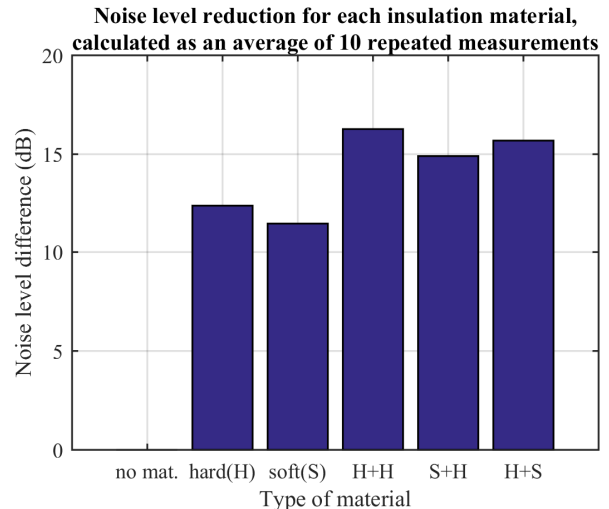
Fig.5. Noise level reduction for different damping materials (taking into account frequency range from 100 Hz to 5 kHz)
