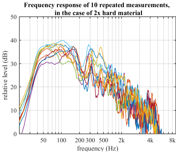
Fig.2e. Spectra of impact noise generated when the metal disk hits the metal plate with damping material (hard + hard) placed on top of the plate (noise levels are given in relative units, that is, dB)
