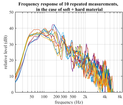
Fig.2e. Spectra of impact noise generated when the metal disk hits the metal plate with damping material (soft + hard) placed on top of the plate (noise levels are given in relative units, that is, dB)
