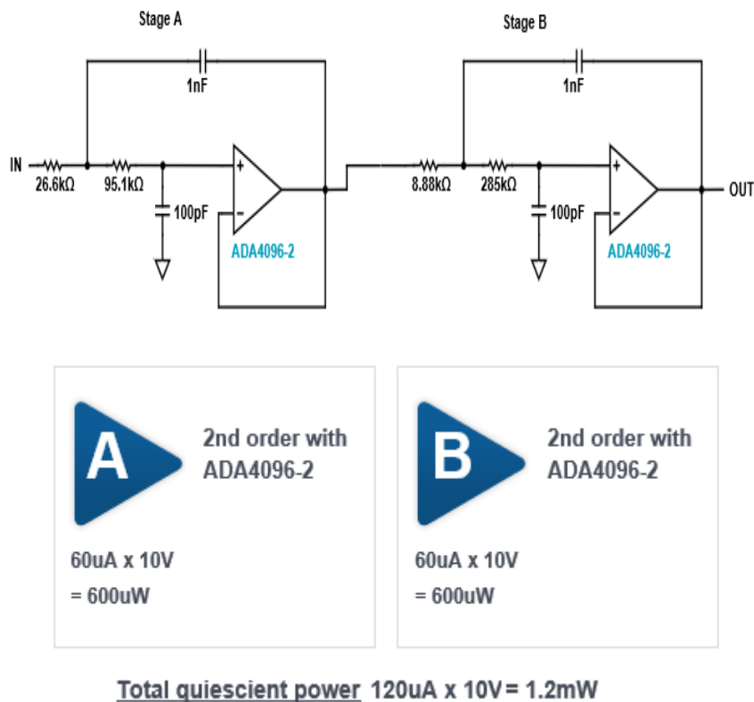
Fig.1. Low pass filter realization in Analog Filter Wizard tool and results from power estimation in the tool
