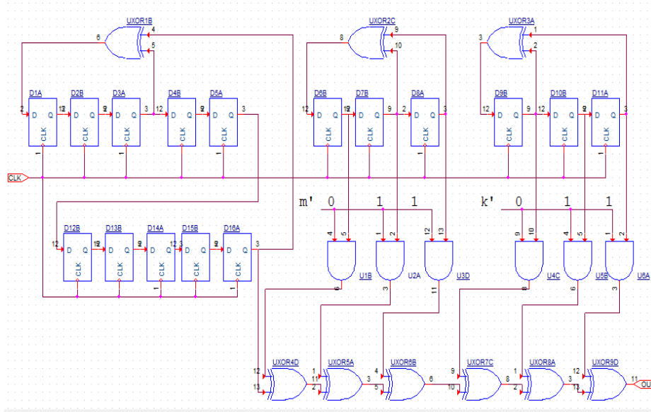
Fig.3. Electrical circuit of Kasami pseudo-random sequence generator
