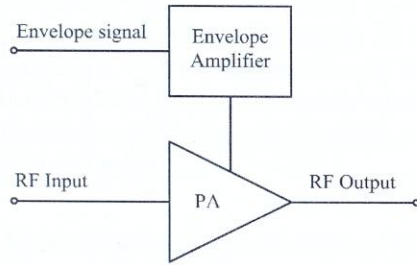
Fig.7. Block diagram of ETPA system.
