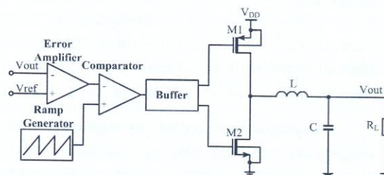
Fig.1. Switching-mode buck dc-dc converter system using PWM control.
