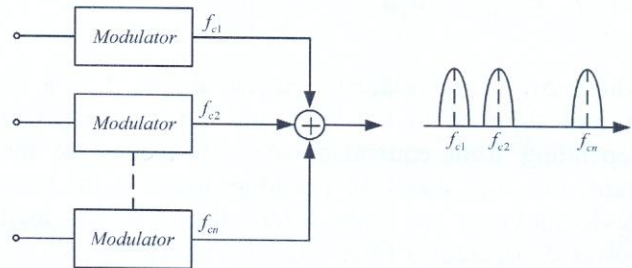
Fig.6. Block circuit diagram of OFDM modulation.
