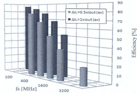
Fig.5. Efficiency of the switching-mode buck dc-dc converter system as function of f_s and \Delta i_L .
