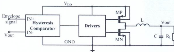
Fig. 5. Hysteresis controlled switching-mode amplifier.
