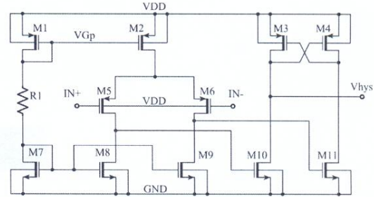
Fig. 6. Comparator with hysteresis.
