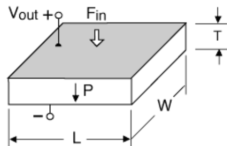
Fig. 1. Single-layer piezoelectric structure [4]
