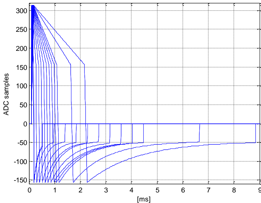
Fig. 1 Illustration of the simulated 13 pacing pulses
