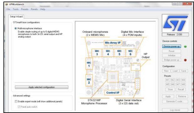
Fig. 10. Microphone selection
