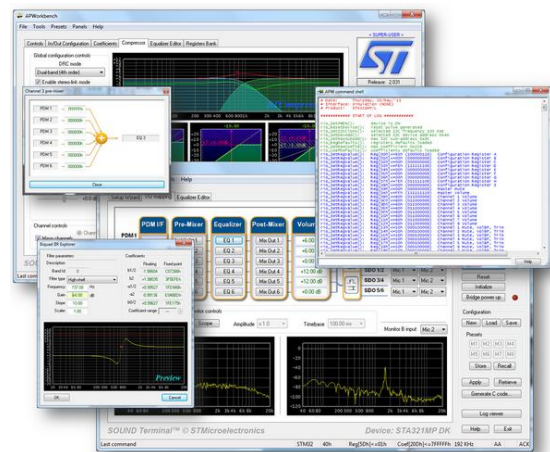
Fig. 8. APWorkbench software
