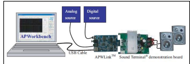
Fig. 2. Block diagram
