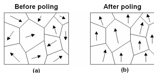
Figure 1: A diagram of domain structure before (a) and after (b) poling.
