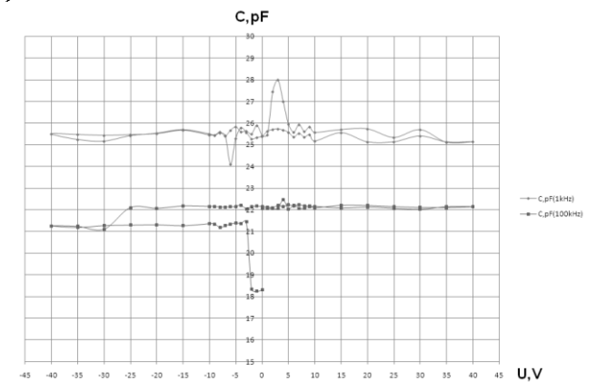
Figure 6: Capacitance-voltage characteristics at 1kHz and 100kHz
