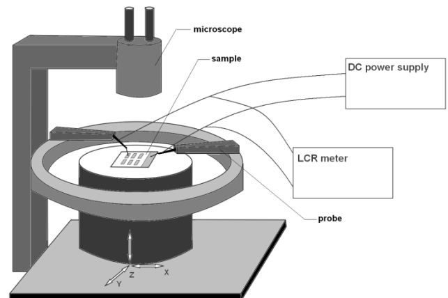
Figure 3: The experimental set for measuring the capacitance-voltage characteristics
