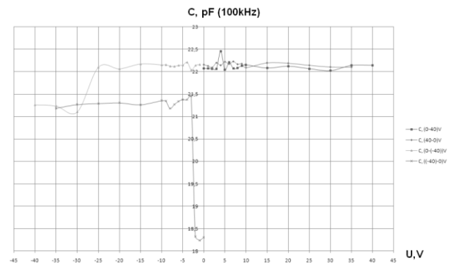
Figure 5: Capacitance-voltage characteristics at 100kHz
