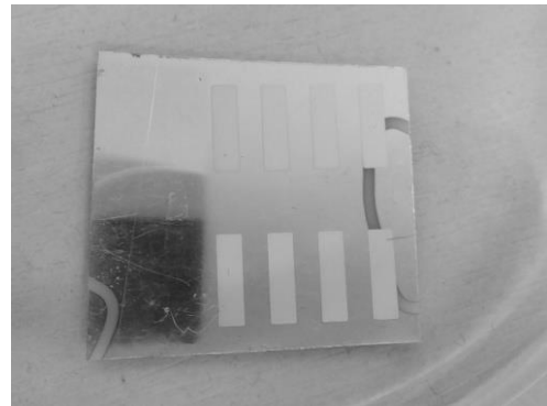
Figure 2: 1\mu\text{m} PVDF layer on PET substrate with Al top and bottom electrodes
