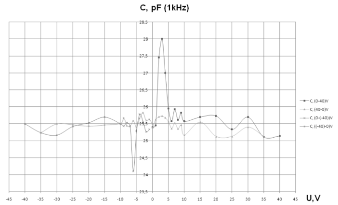
Figure 4: Capacitance-voltage characteristics at 1kHz
