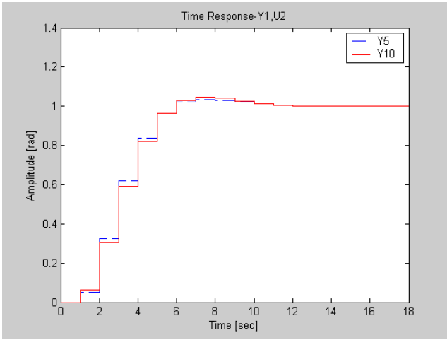
Fig.2. Transient closed-loop system response u_2 = T_m v.s. y_1 = \delta , full order – red and reduced order - blue.
