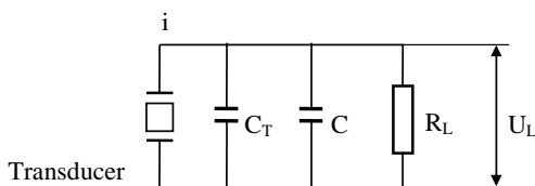
Fig.3 Equivalent replacement scheme
